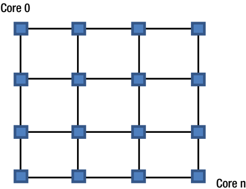
Figure 5-2. 2D mesh network
