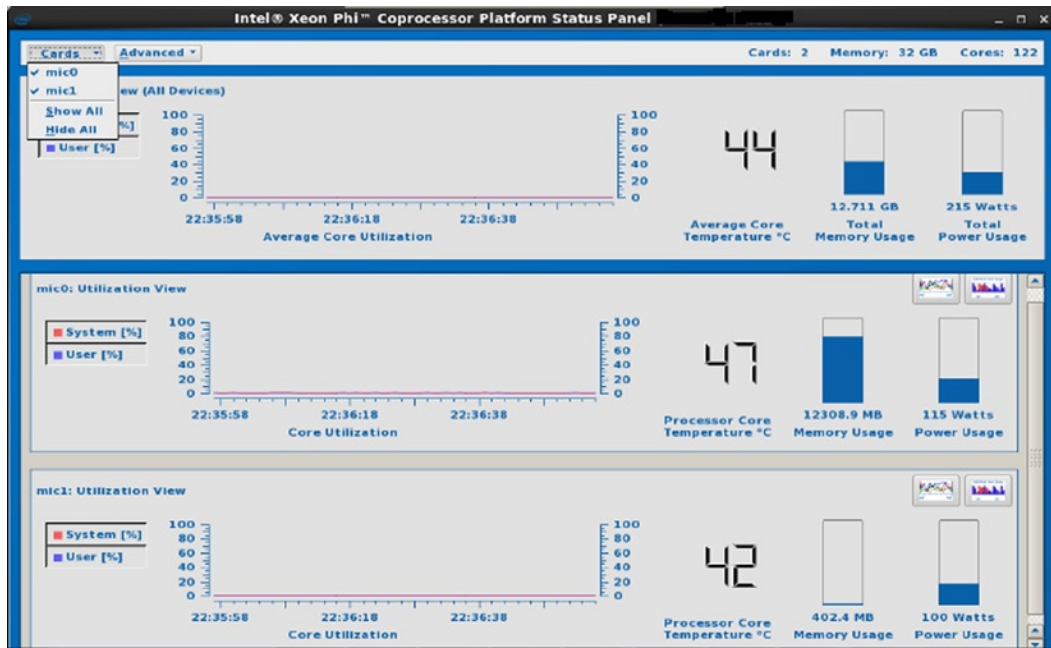
Figure 12-2. MicSmc GUI mode execution with two cards available on the system
