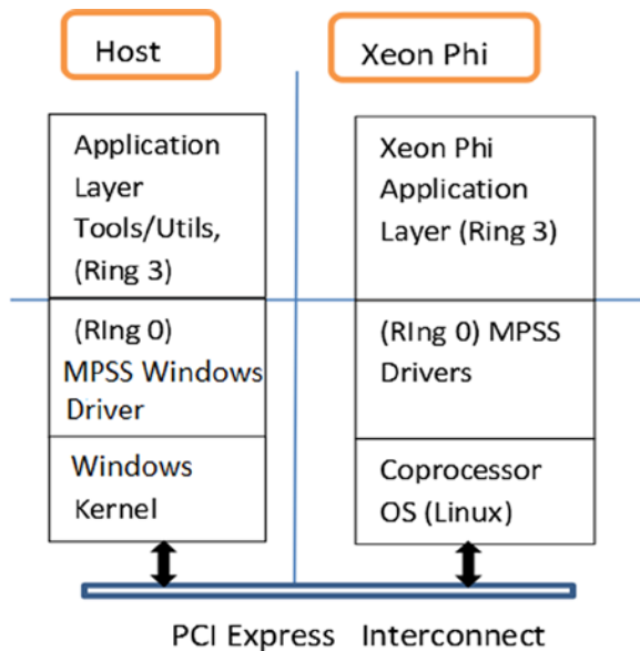
Figure 12-1. System components in the Microsoft Windows environment
