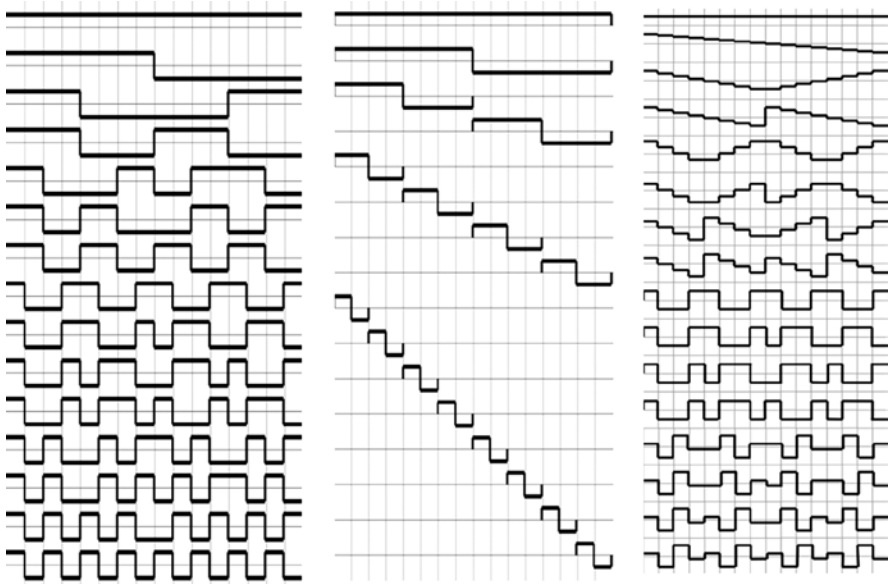
Figure 3-21. (Left) Walsh Hadaard basis set. (Center) HAAR basis set. (Right) Slant basis set
