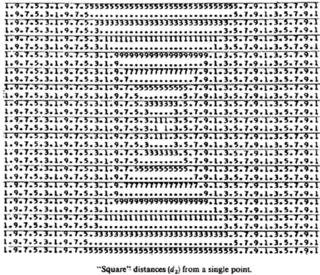
Figure 4-3. An early Rosenfeld and Pfaltz rendering that illustrates a distance function (square distance in this case) using a line printer as the output device. (Image © reprinted from Rosenfeld and Pfaltz, Pattern Recognition (Oxford: Pergamon Press, 1968), 1:33-61. Used with permission from Elsevier)
