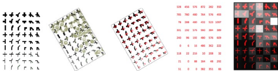
Figure A-26. Method of computing and binning detected alphabet features across rotated image sets, mocked-up SIFT data for illustration. (Left) Original image. (Center left) Rotated image annotated with detected points. (Center) Count of all detected points across entire image superimposed on alphabet cell regions. (Center right) Summary bin counts of detected alphabet features in grid cells. (Right) 2D histogram rendering of bin counts as an image; each pixel value is the bin count. Brighter pixels in the image have a higher bin count, meaning that the alphabet cell has a higher detection count
