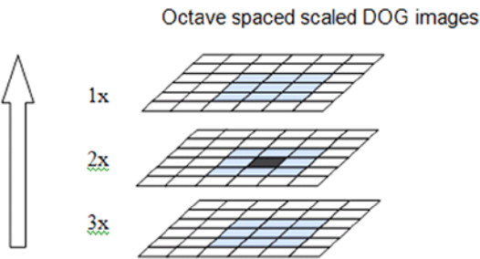
Figure 6-16. SIFT interest point or keypoint detection using scale invariant extrema detection, where the dark pixel in the middle octave is compared within a 3x3x3 area against its 26 neighbors in adjacent DOG octaves, which includes the eight neighbors at the local scale plus the nine neighbors at adjacent octave scales (up or down)
