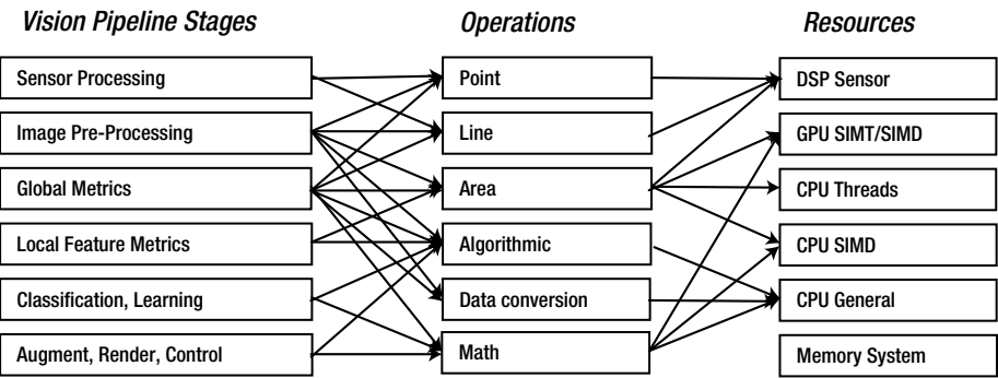
Figure 8-1. Hypothetical assignment of vision pipeline stages to operations and to compute resources. Depending on the actual resource capabilities and optimization targets for power and performance, the assignments will vary
