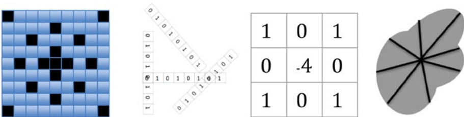
Figure 4-8. illustrating various descriptor patterns and shapes. (Left) Sparse. (Center left) Nets or strips. (Center right) Kernels. (Right) Radial spokes
