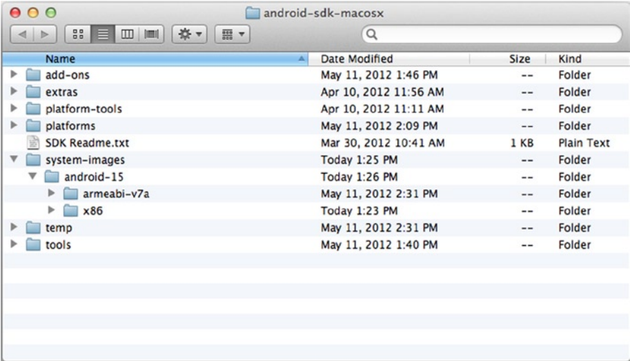
Figure 6-22. API Level 15
