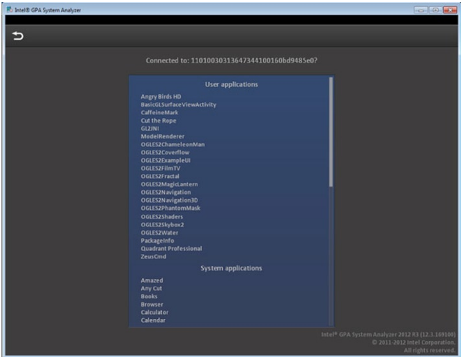
Figure 8-28. Applications List
