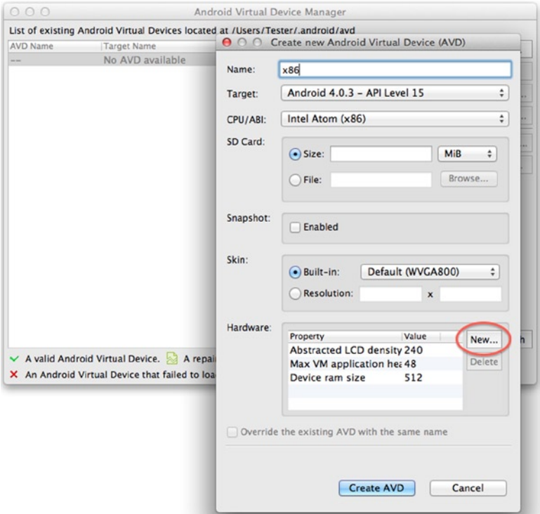
Figure 6-24. Hardware Section
