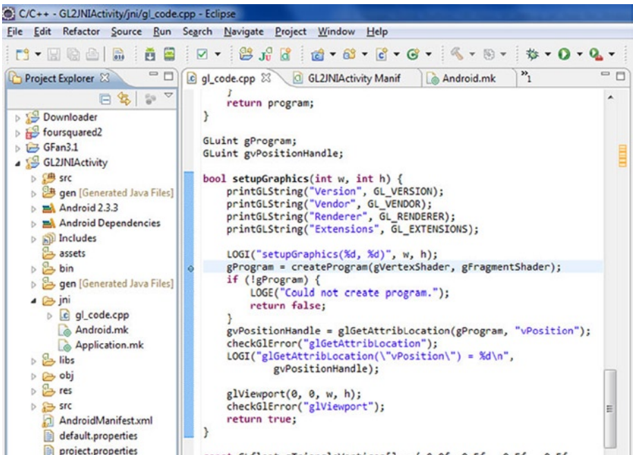
Figure 8-26. Setting Breakpoints
