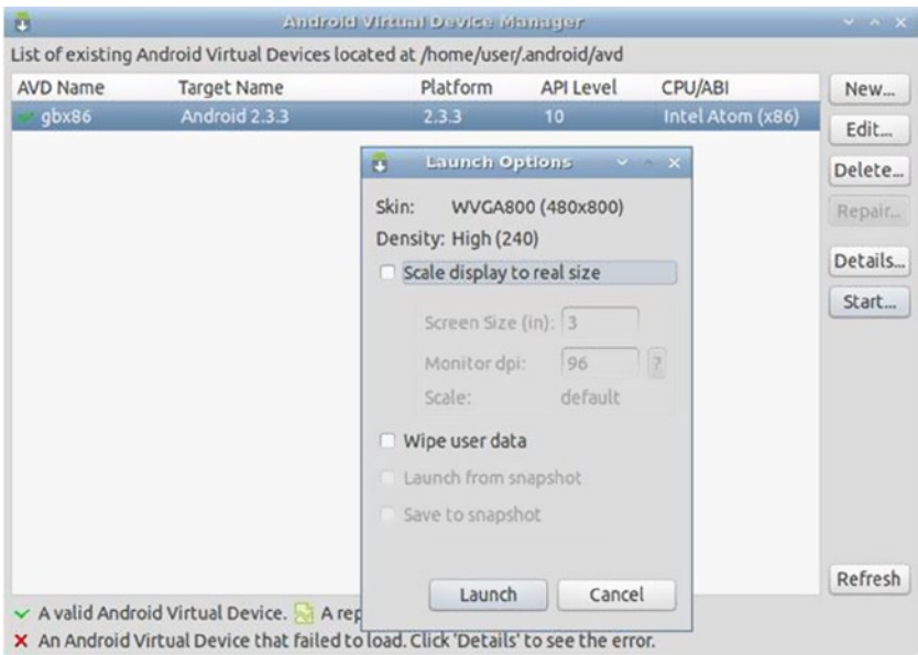
Figure 6-12. Launch Options
