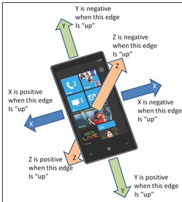
Figure 7-2: Accelerometer orientation
