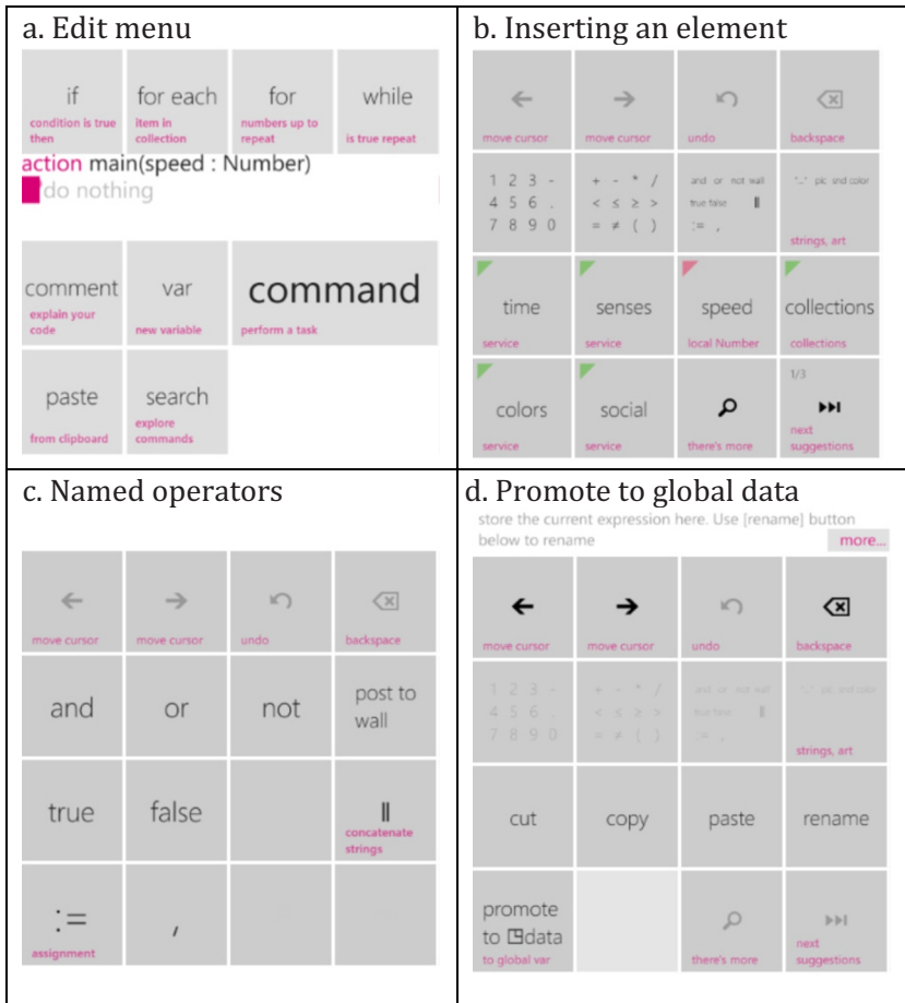
Figure A-3: Editing the first line
