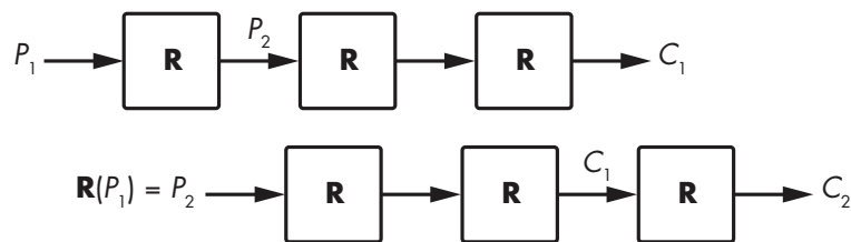
Figure 4-1: Principle of the slide attack, against block ciphers with identical rounds
