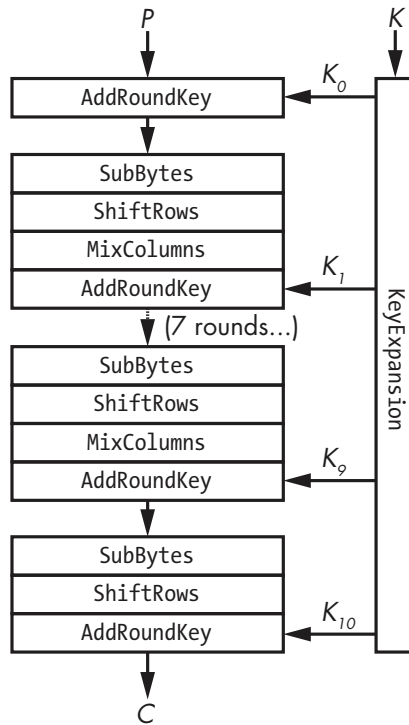
Figure 4-4: The internal operations of AES
