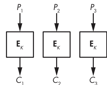
Figure 4-6: The ECB mode
