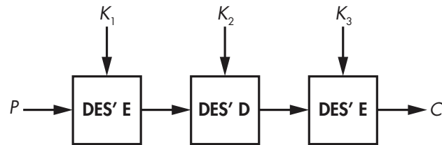
Figure 4-11: The 3DES block cipher construction
