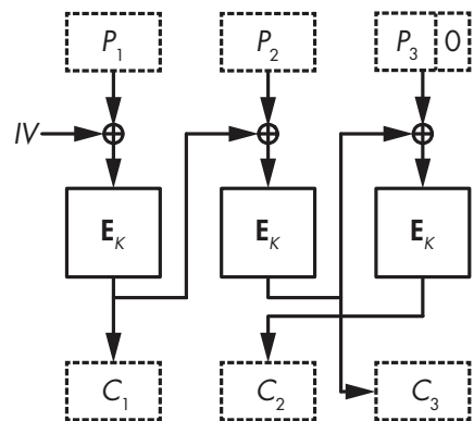
Figure 4-9: Ciphertext stealing for CBC-mode encryption
