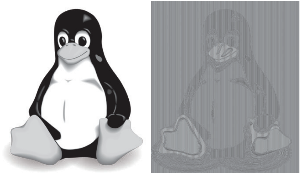
Figure 4-7: Original image (left) and ECB-encrypted image (right)
