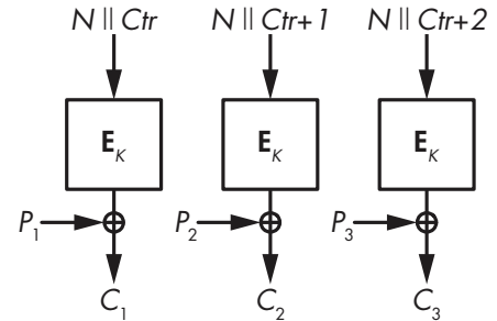
Figure 4-10: CTR mode
