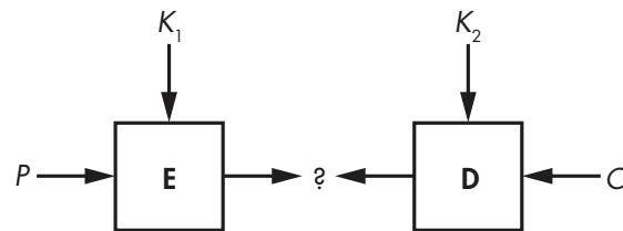
Figure 4-12: Meet-in-the-middle attack
