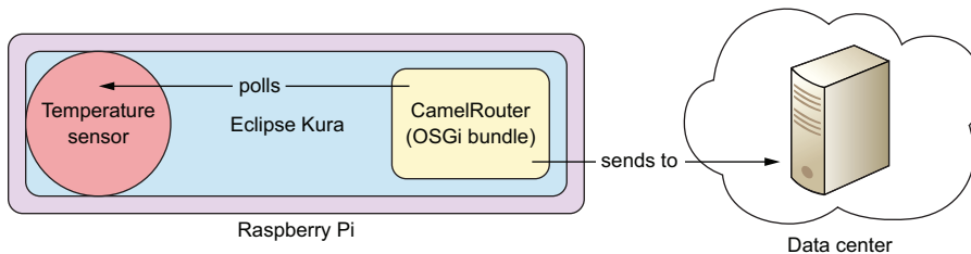
Figure 21.5 Apache Camel and Eclipse Kura integration architecture
