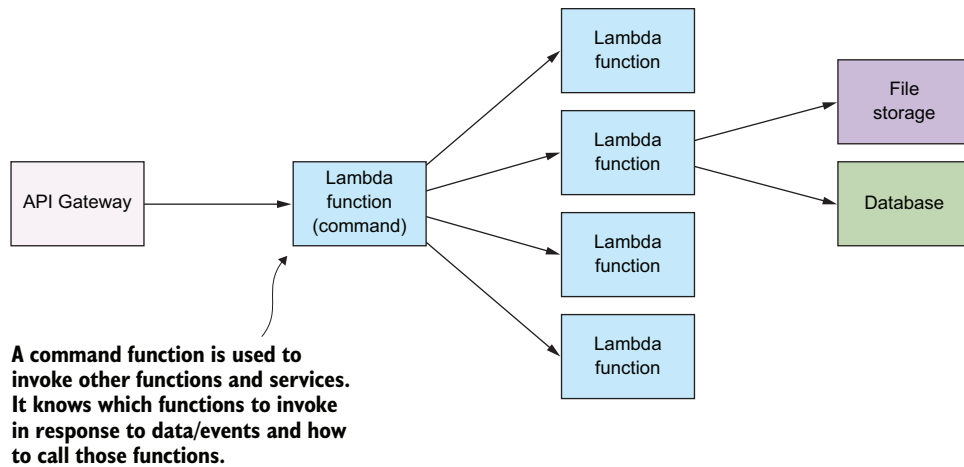
Figure 2.12 The command pattern is used to invoke and control functions and services from a single function.
