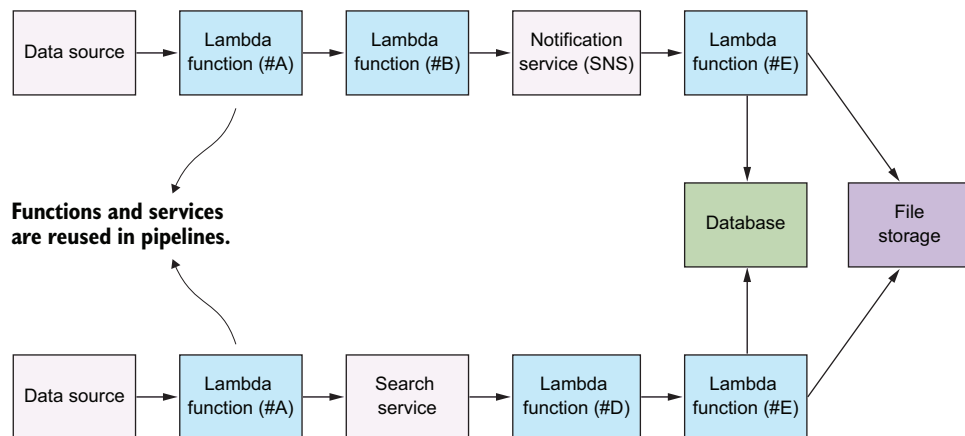
Figure 2.17 This pattern encourages the construction of pipelines to pass and transform data from its origin (pump) to its destination (sink).
