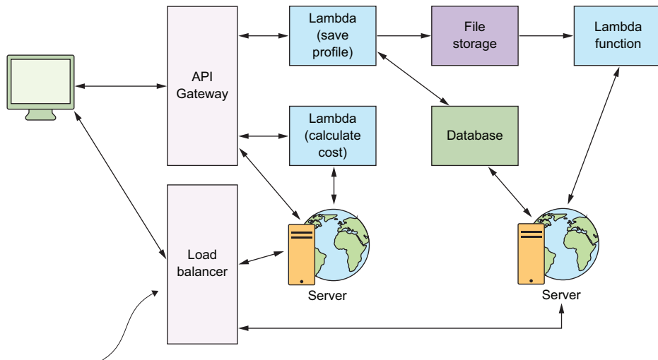
Figure 2.6 The hybrid approach is useful if you have a legacy system that uses servers.
