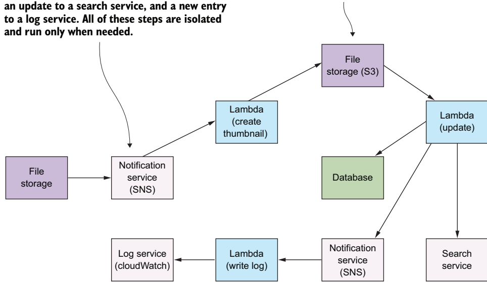
Figure 2.9 The compute-as-glue architecture uses Lambda functions to connect different services and APIs to achieve a task.
