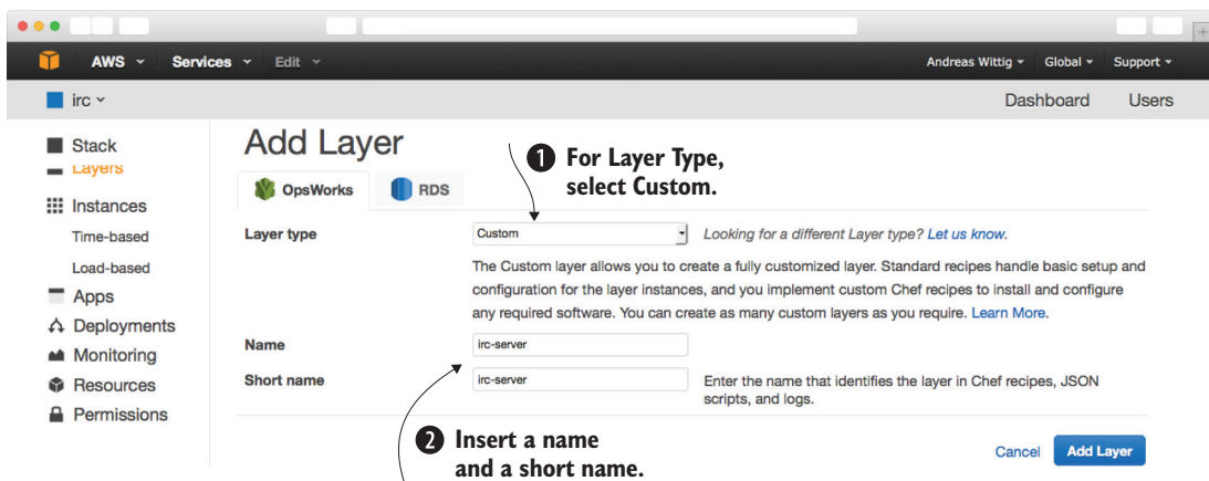
Figure 5.11 Creating a custom layer to deploy an IRC server
