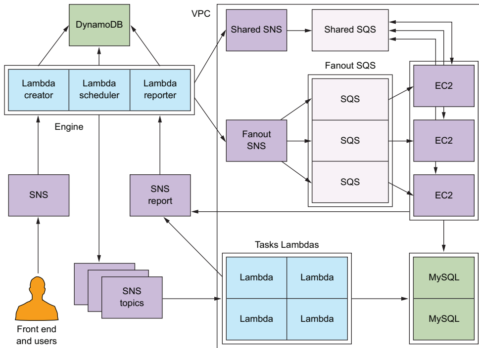
Figure 2.7 The Hybrid-Serverless Job-Processing System designed by EPX Labs
