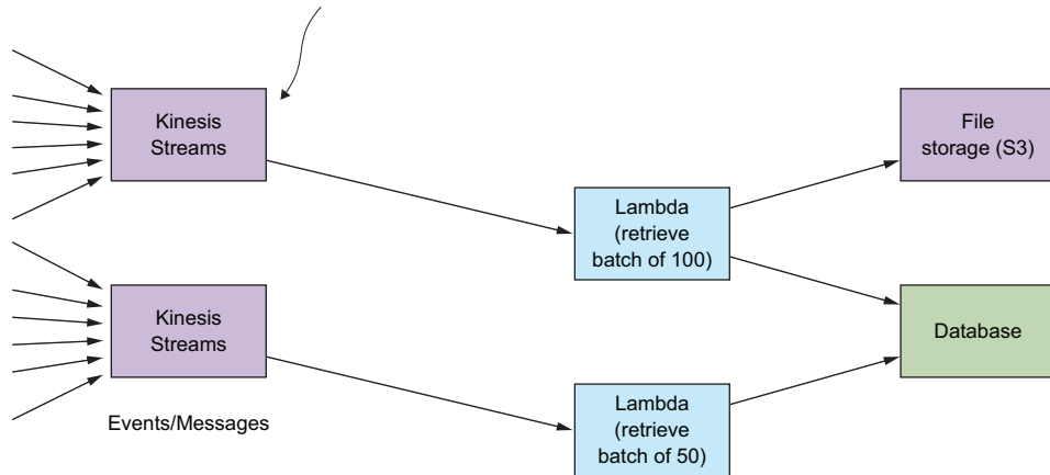
Figure 2.11 Lambda is a perfect tool to process data in near real time.
