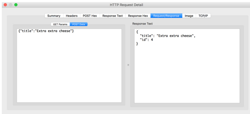
Figure 2.15 HTTPSCOOP POST request/response. The only field needed to create a new topping is the title, and it's set to Extra extra cheese (yum!). The response shows the ID and title—the entire representation—of the newly added item.
