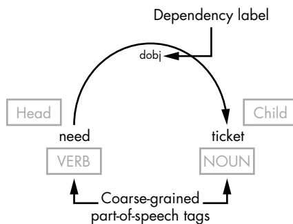
Figure 2-3: A graphical representation of a syntactic dependency arc
